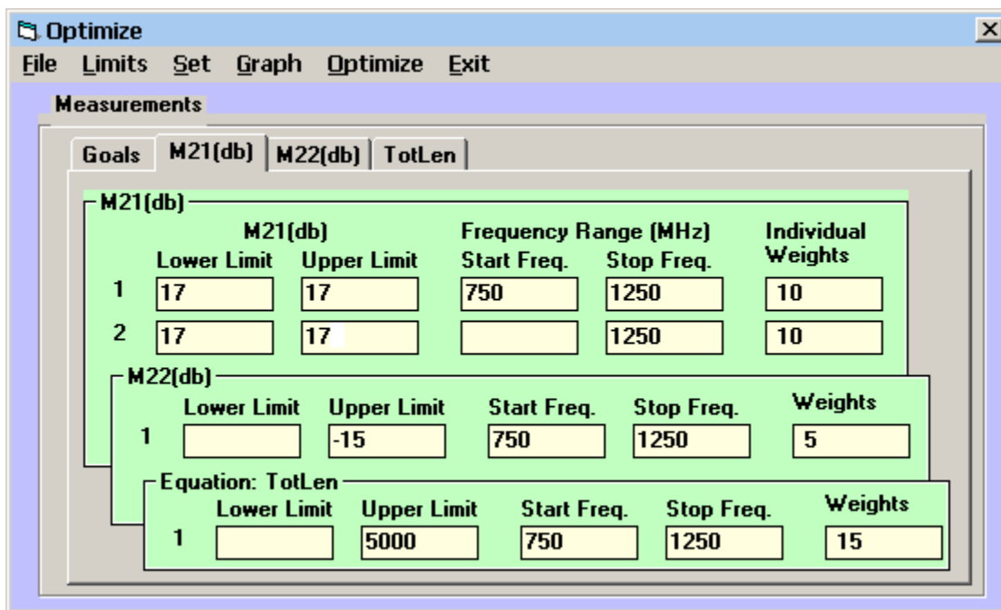
Figure 10, Setting LINC2 Optimizer Goals and Weights
