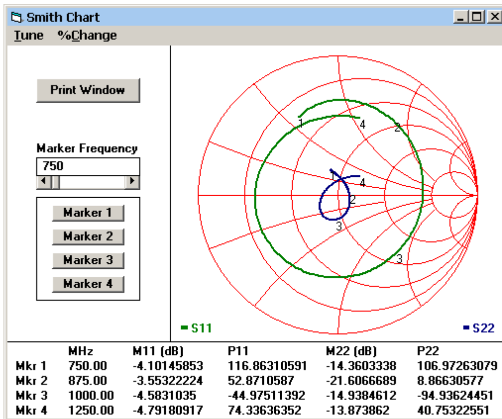
Figure 13, LINC2 Optimized S22 (S11 not Optimized)
