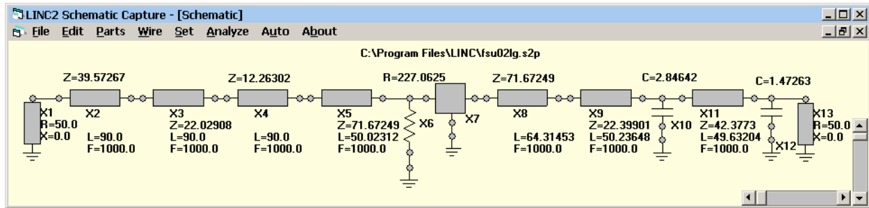
Figure 5, LINC2 Synthesized Amplifier Schematic
